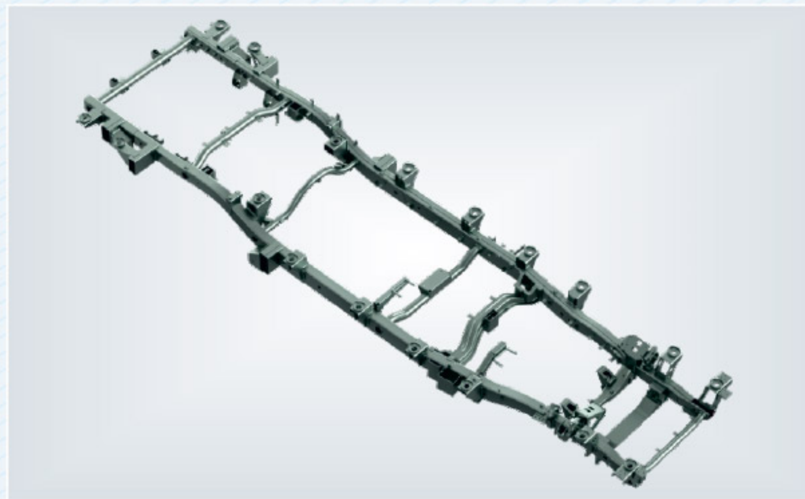
All-New C-IN-C Chassis Rectangular type, Excellent Bending Strength & Torsional Rigidity
